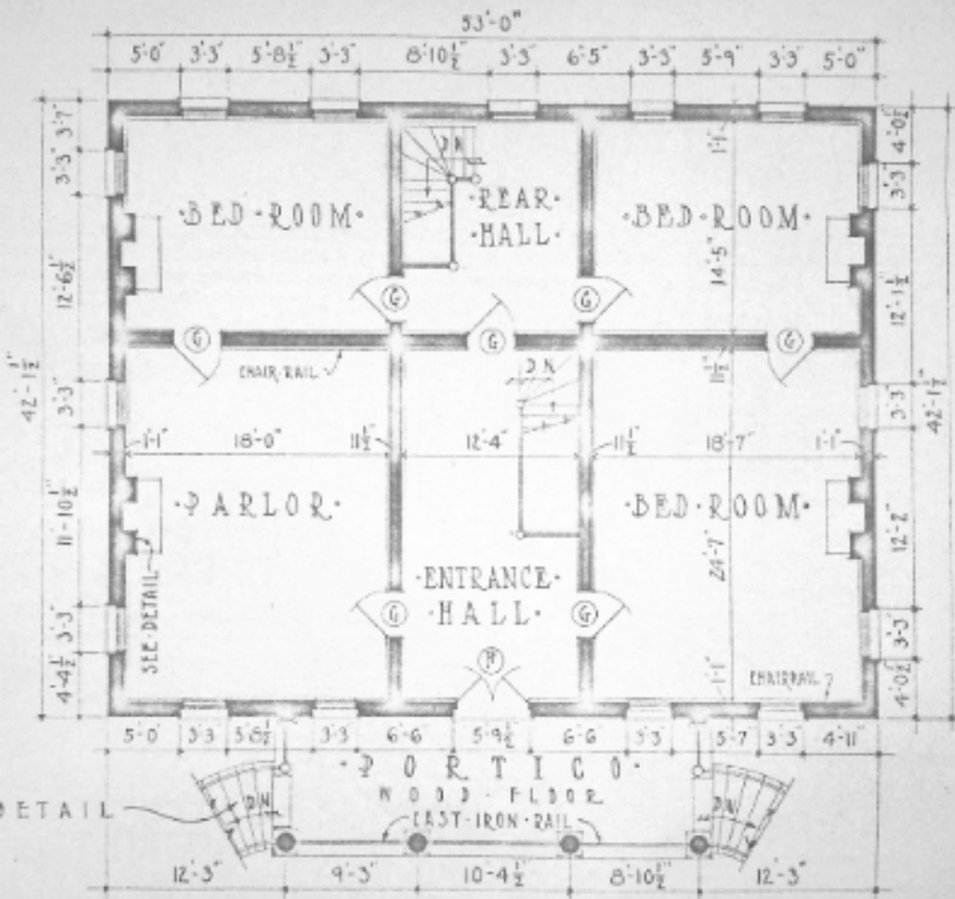
MAIN FLOOR PLAN SCALE 1/8" = 1'-0"
